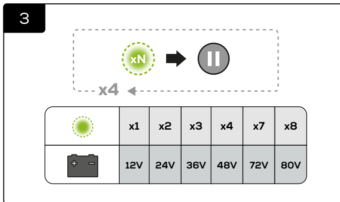
A number of green flashes followed by a pause is repeated four times. The number of flashes indicates the voltage detected.
